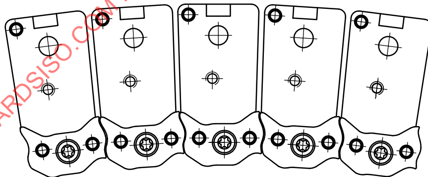
Figure 12 — Sinker cam box
