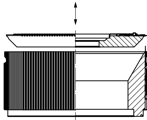
b) Vertical adjustment of the needle disc
