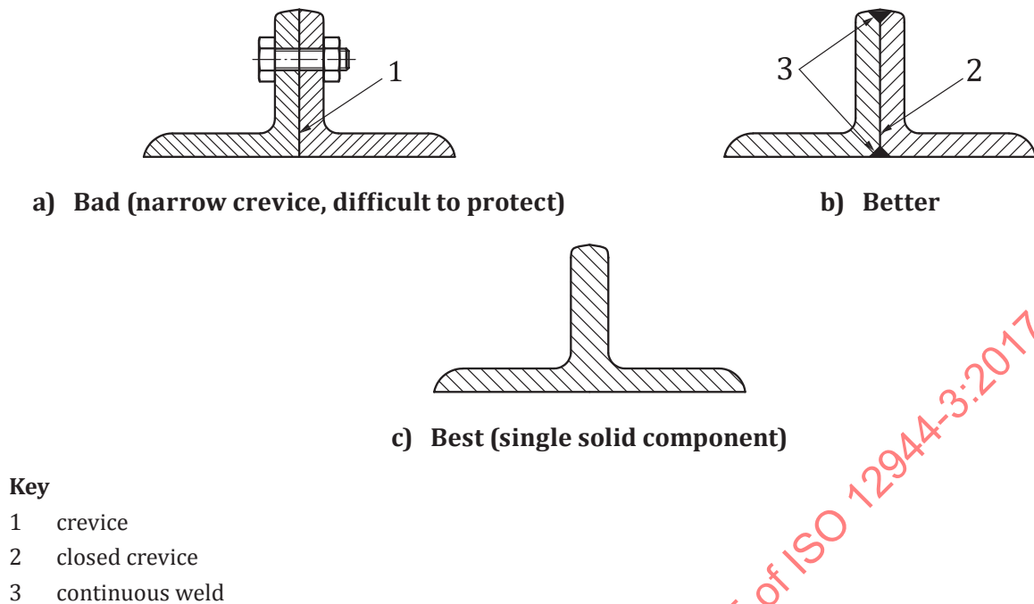
Figure D.3 — Treatment of gaps
