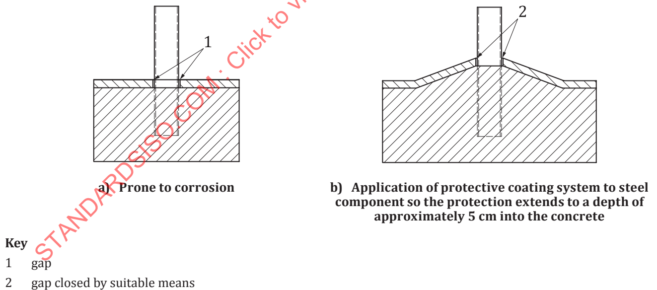
Figure D.4 — Composite steel/concrete structure
