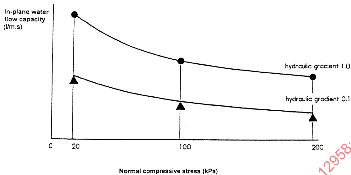
Figure 3: Typical examples of in-plane water flow capacity curves
