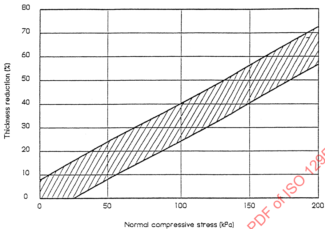
Figure 1: Compression-deflection envelope of the elastomeric closed-cell foam rubber
