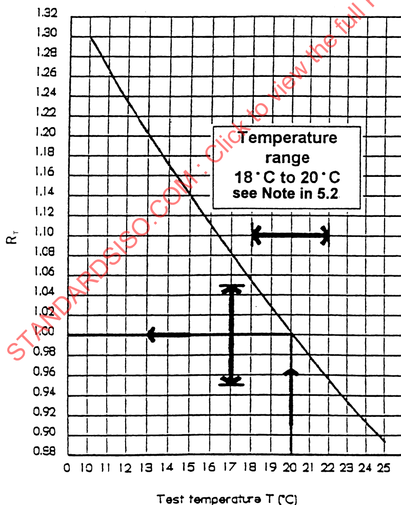
Figure A.1: Graphical presentation of the correction factor R_T
