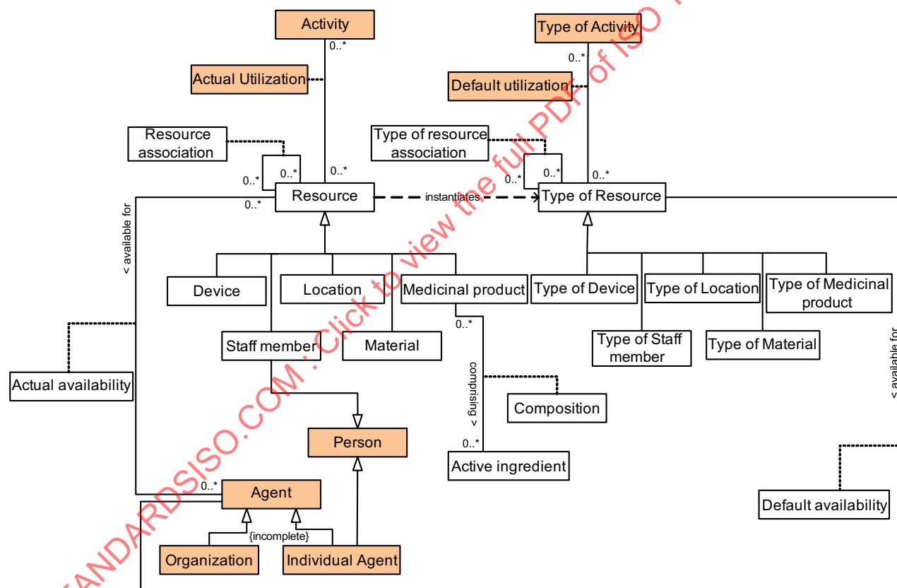
Figure 10 — UML model for resource management Objects
