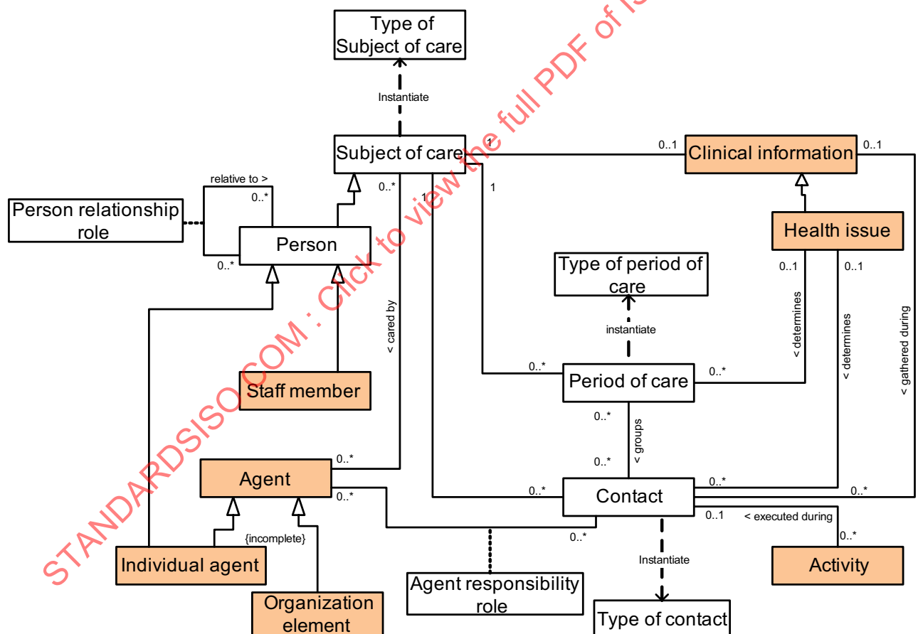
Figure 7 — UML model for subject of care objects
