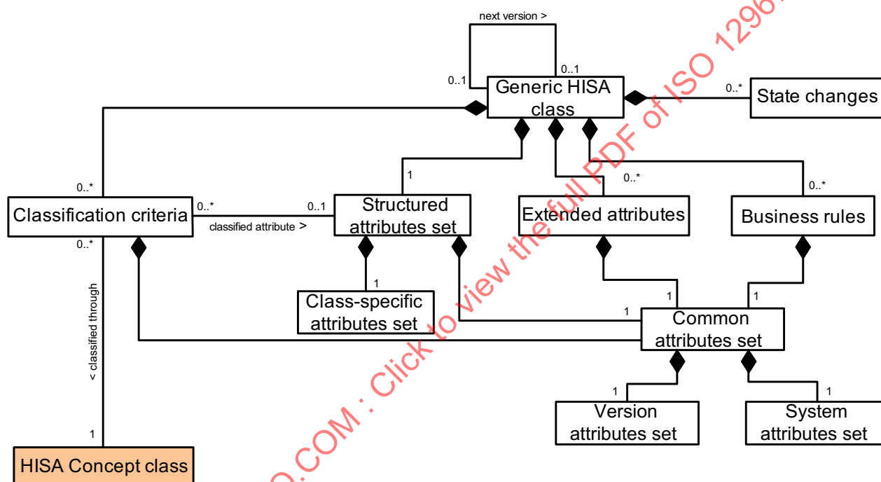
Figure 5 — The generic HISA class
