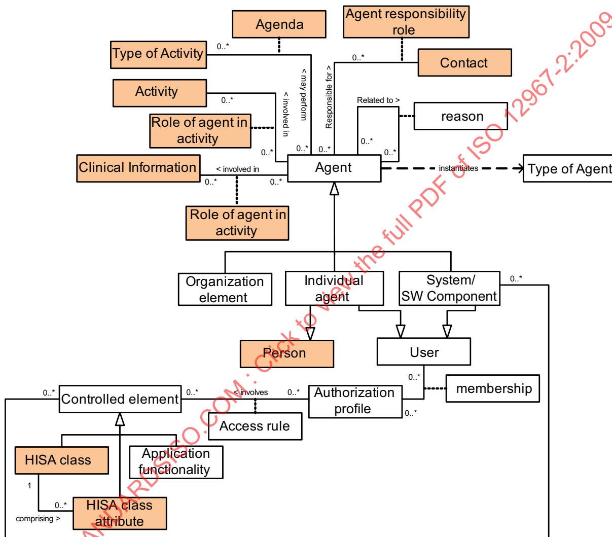
Figure 11 — UML model for Users and Authorization Objects
