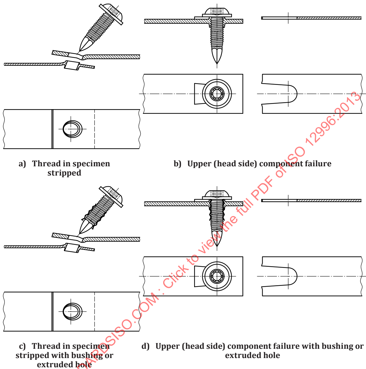
Figure A.4 — Typical failure modes of screw joints (machine screw or tapping screws)
