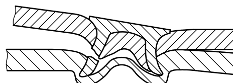
c) Failure of the specimen material
