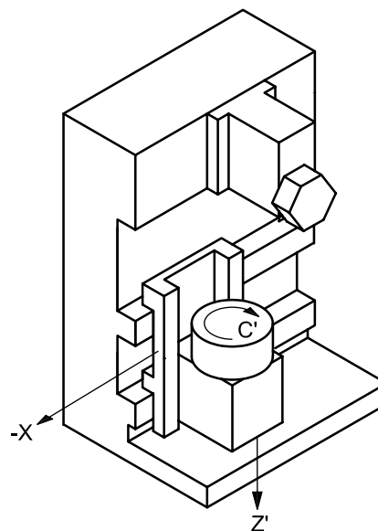
d) Compound workholding spindle type
