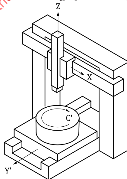
d) Fixed column (portal type), moving workholding spindle (Y-axis) V [w C' Y' b X Z t]
