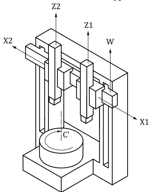
a) Fixed column (portal type), moving cross-rail V [w C' b W X1 Z1 t 1 ] V [w C' b W X2 Z2 t 2 ]
