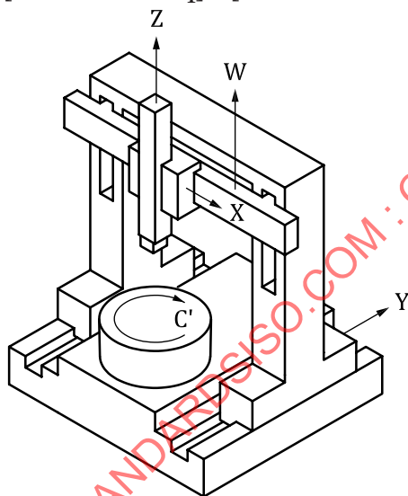
a) Fixed column (portal type), moving cross-rail V [w C' b W X1 Z1 t 1 ] V [w C' b W X2 Z2 t 2 ]
