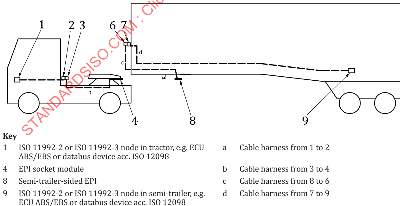
Figure 3 — Example of an electrical wiring diagram of FACS equipped tractor and semi-trailer
