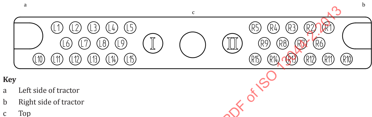
Figure B.1 — Contact allocation — Rear view of socket, tractor side
