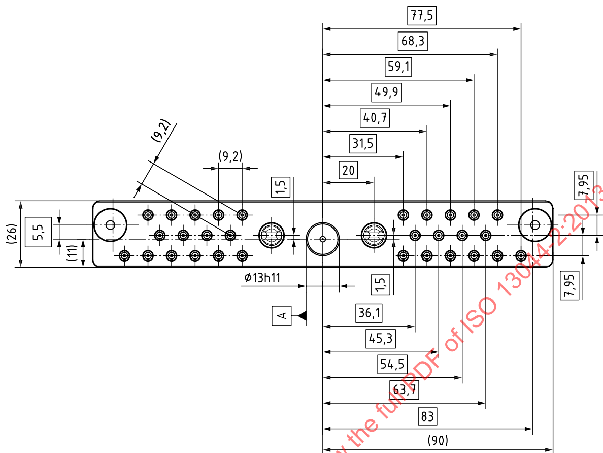
c) Dimensions — Front view
