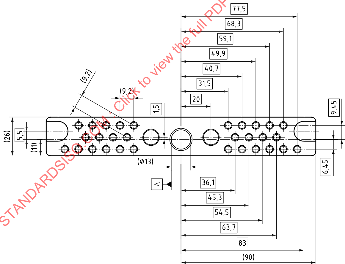
b) Dimensions — Socket front view
