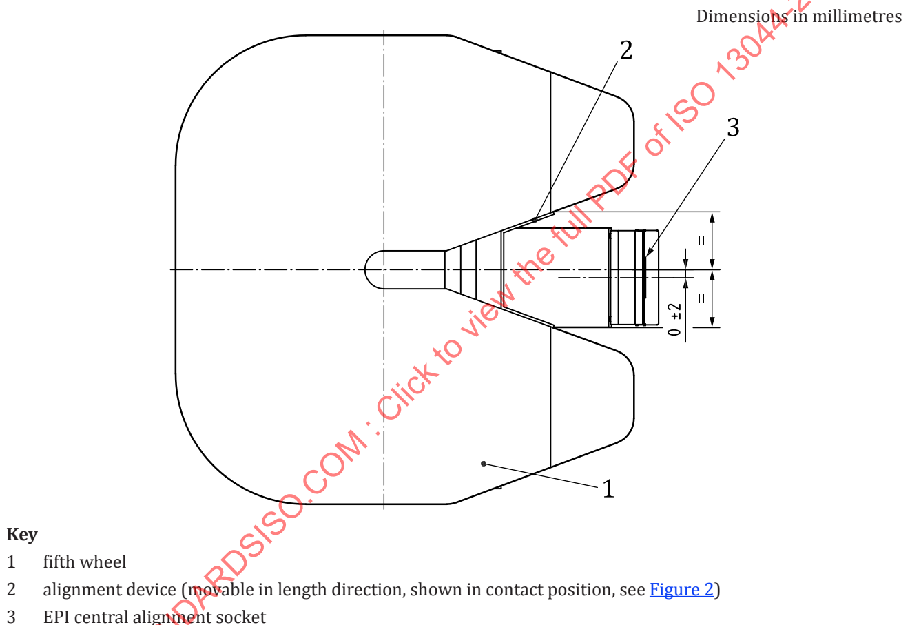
Figure 1 — EPI female module positioning tolerance (displaced shown)
