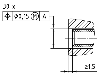
c) Dimensions of female contacts (taken from ISO 7638-1)
