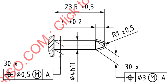
d) Dimensions of male contacts (taken from ISO 7638-1)
