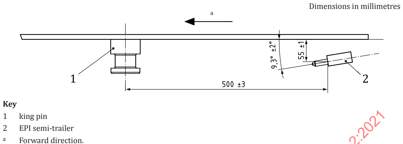
Figure A.3 — Position of the EPI plug module
