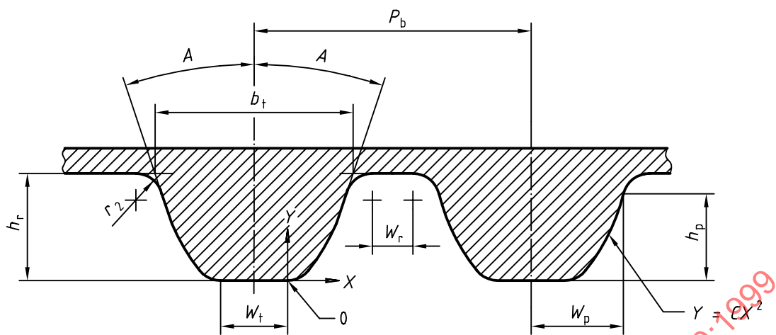
Figure 11 — Pulley generating tool rack form
