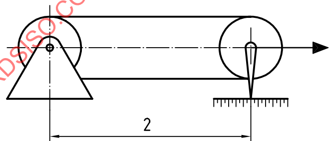
Figure 9 — Clearance between measuring pulley and belt — R-type profile
