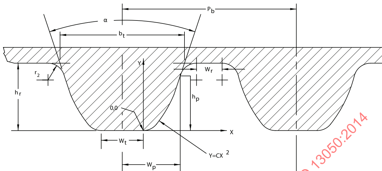
Figure 16 — Pulley generating tool rack form
