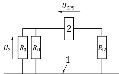
b) Addition of R_0 and measurement of U_2
