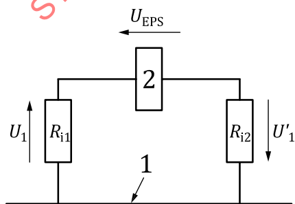
a) Measurement of U_1 and U'_1
