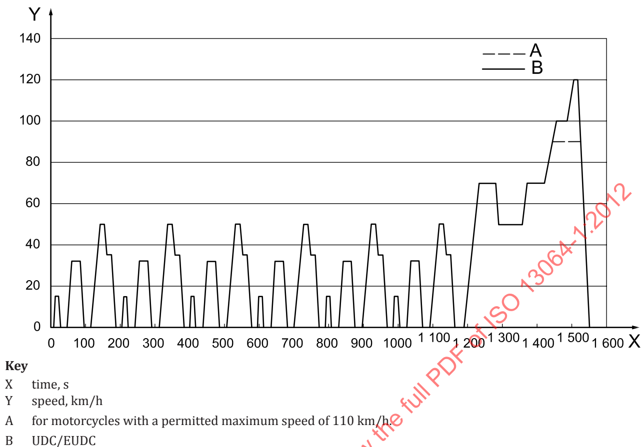
Figure B.1 — Test sequence composition
