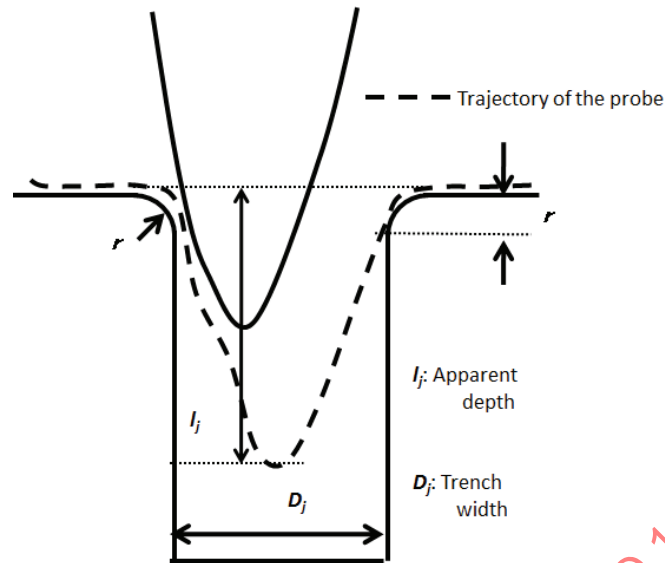
a) Schematic drawing of the probe and the j_{th} trench with the trajectory of the probe apex
