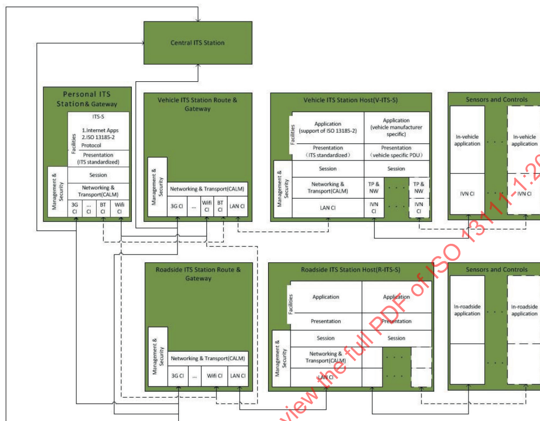
Figure 3 — Connection between P-ITS-S and the other ITS-S based on CALM architecture
