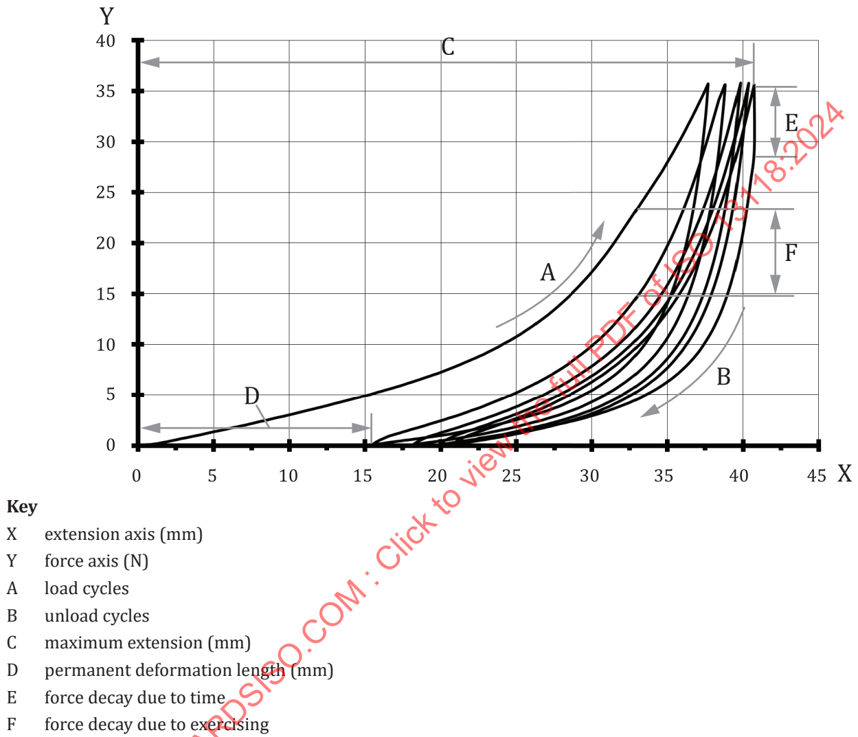
Figure A.1 — Example of a typical cycling graph
