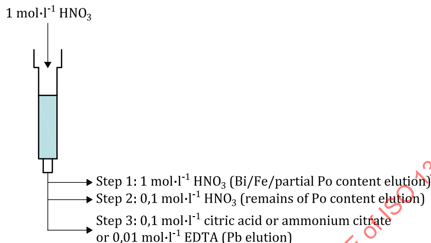
Figure 3 — Separation scheme of ^{210}\text{Pb} with \text{HNO}_3 as starting solution
