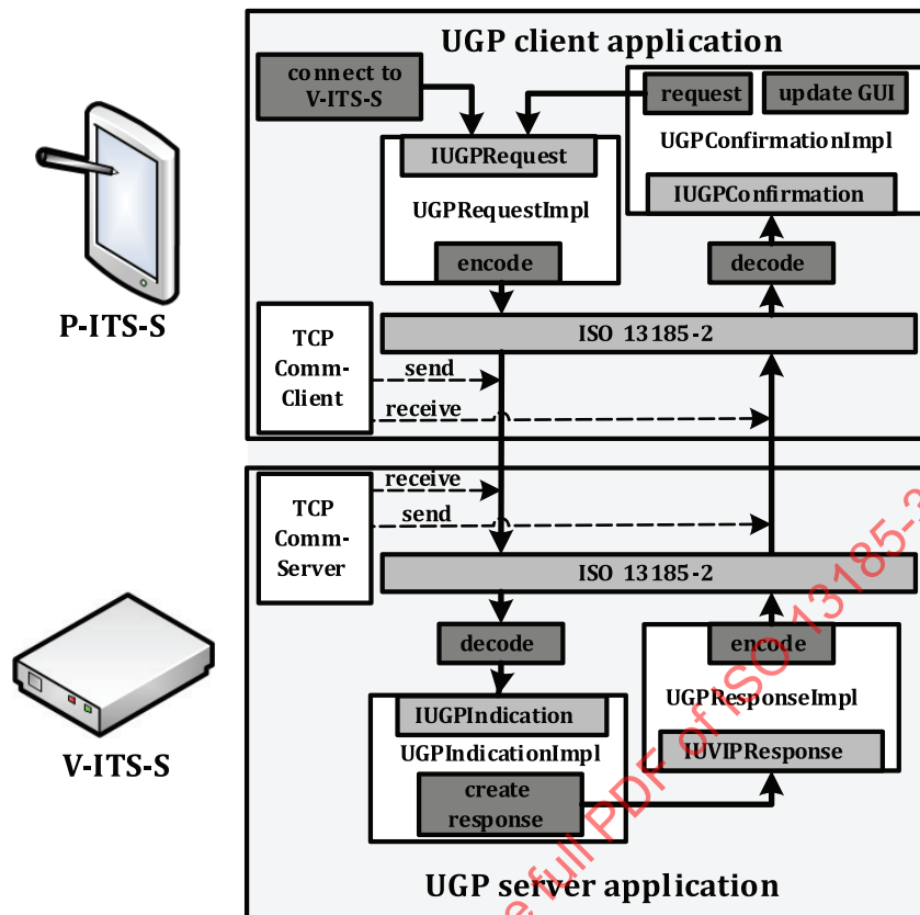
Figure 3 — UGP client and server architecture
