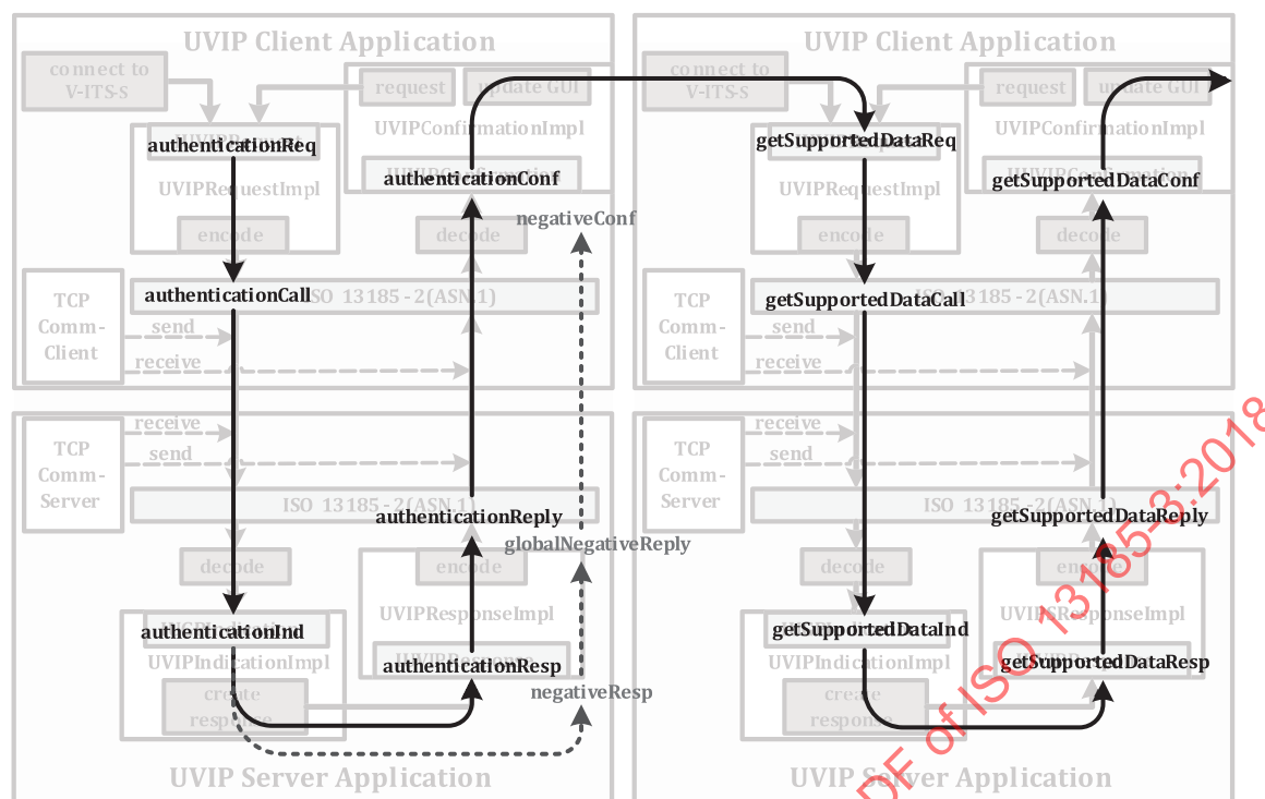
Figure 4 — UGP communication flow
