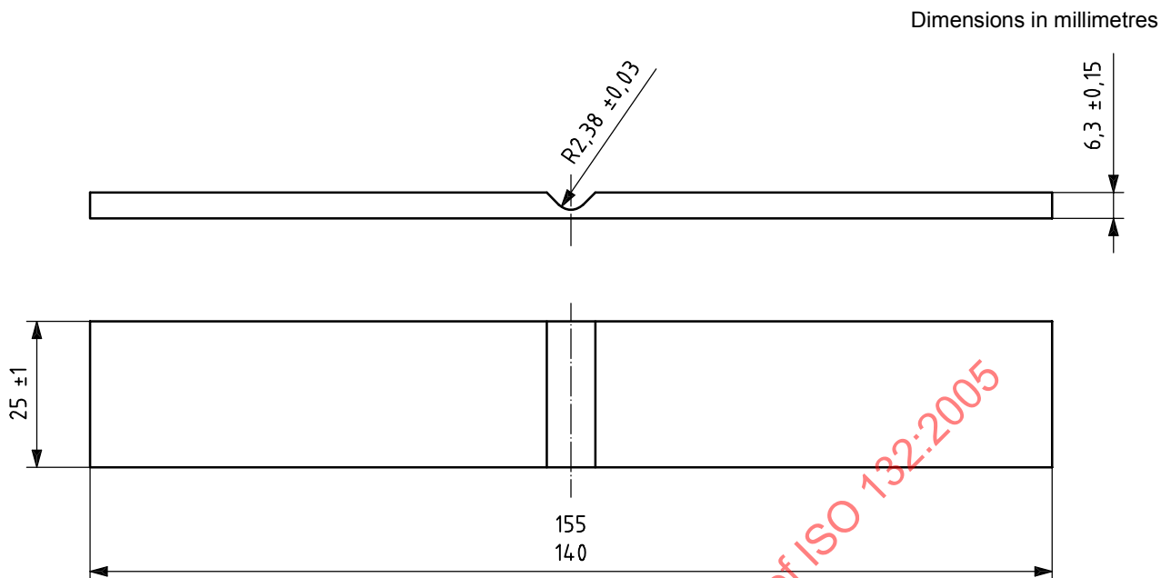
Figure 2 — Test piece
