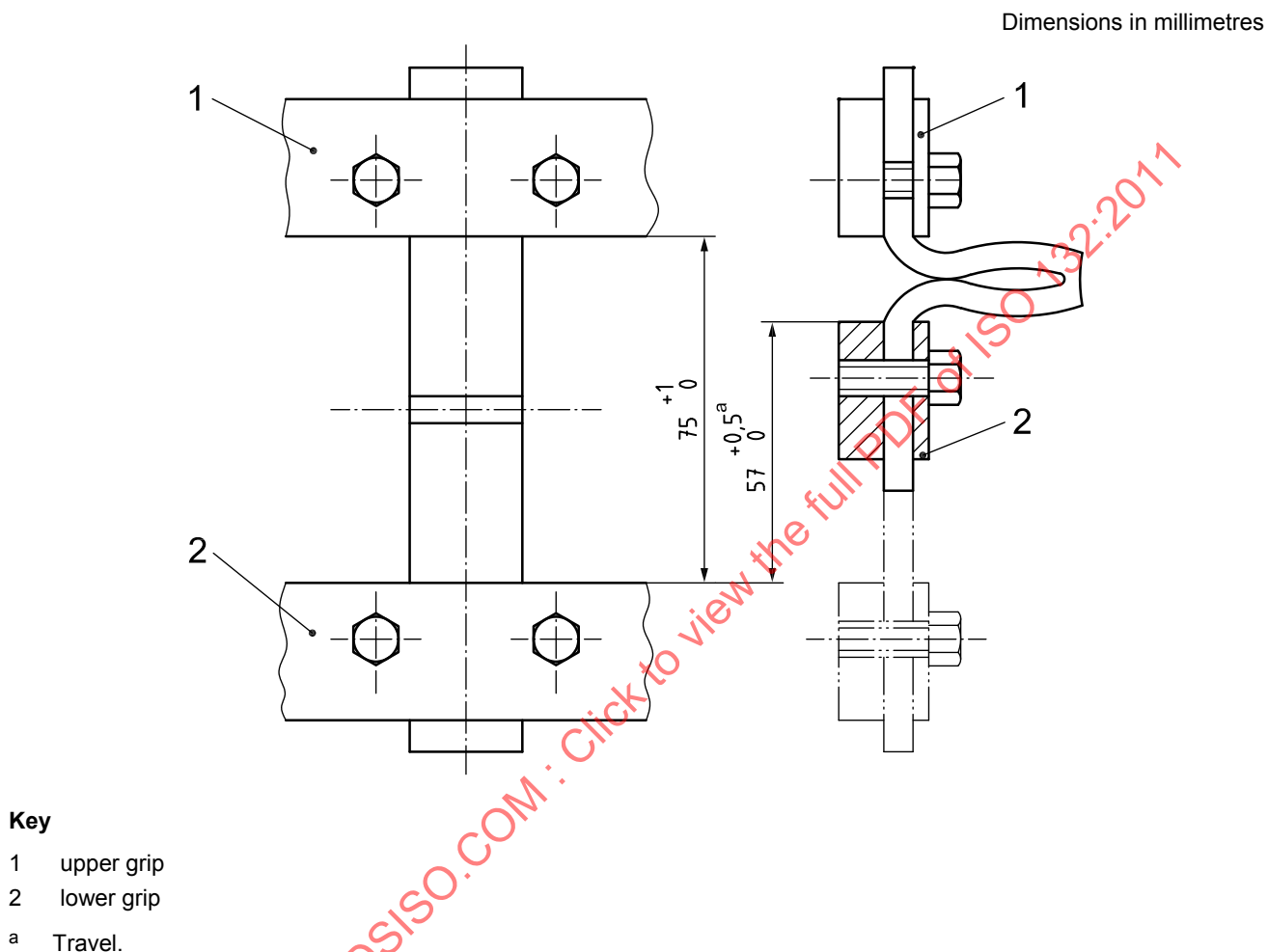
Figure 1 — De Mattia type machine
