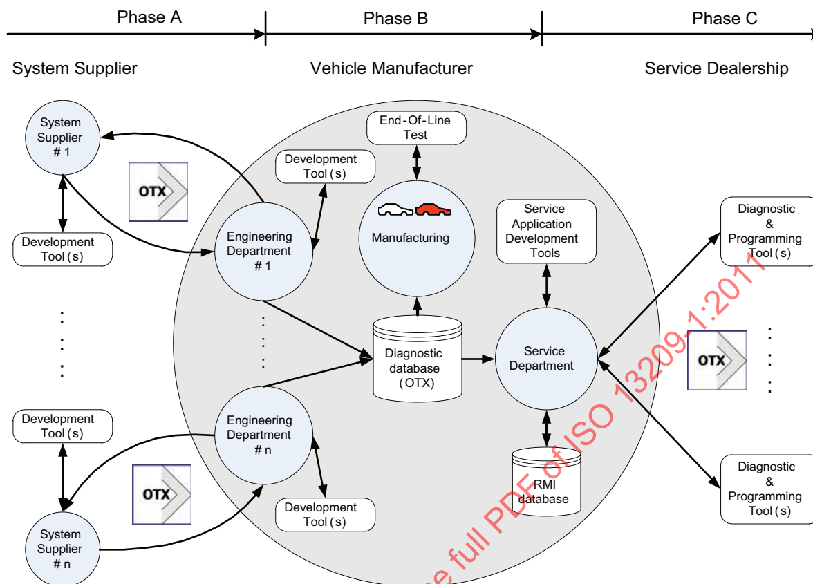
Figure 3 — Example of an OTX process chain
