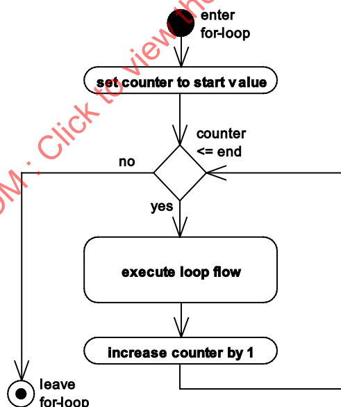
Figure 29 — Behavioural description: for-loop
