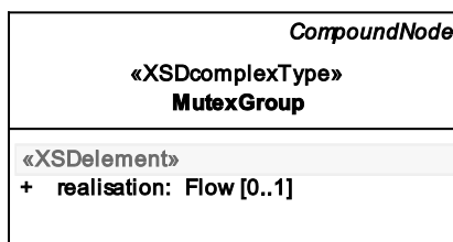
Figure 35 — Data model view: MutexGroup
