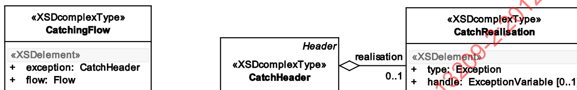
Figure 38 — Data model view: CatchingFlow
