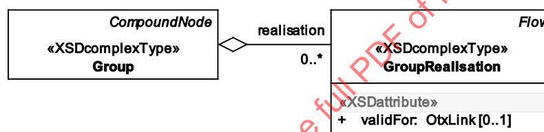
Figure 25 — Data model view: Group
