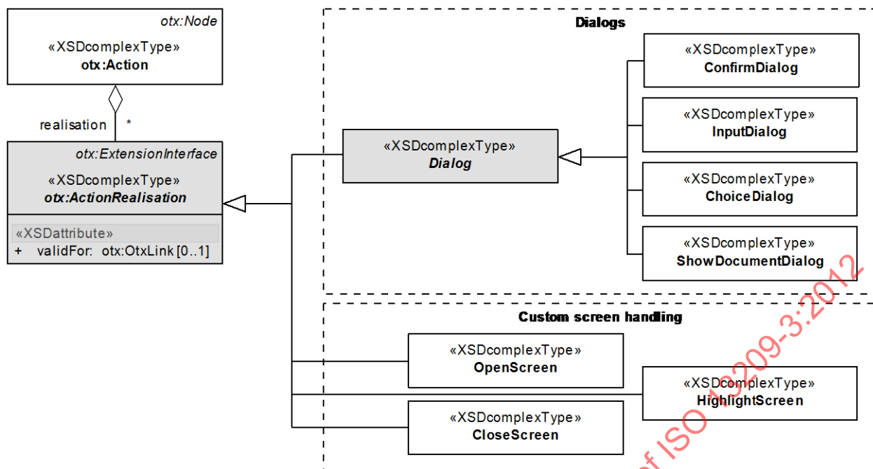
Figure 62 — Data model view: HMI actions overview
