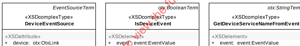
Figure 93 — Data model view: Event related terms
