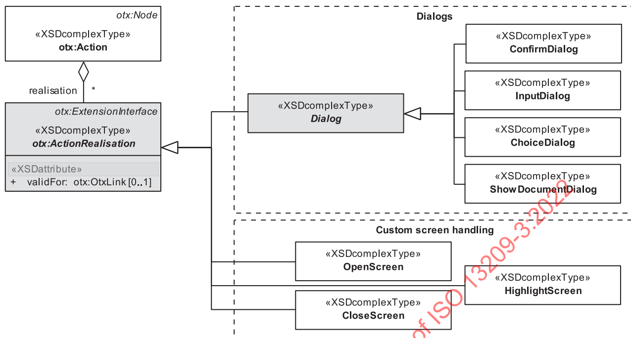
Figure 63 — Data model view: HMI actions overview
