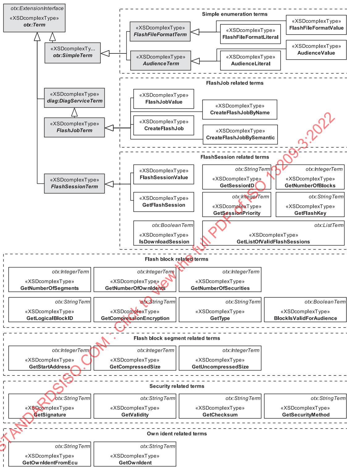
Figure 49 — Data model view: Flash term categories
