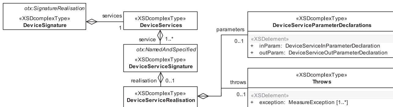
Figure 87 — Data model view: Measure signatures
