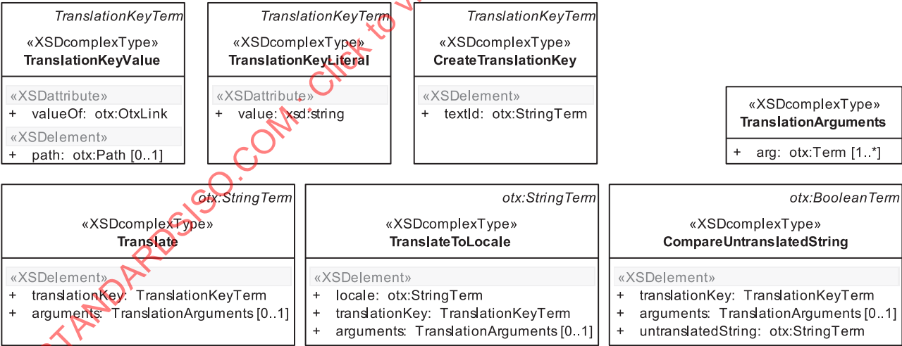
Figure 77 — Data model view: Translation related terms
