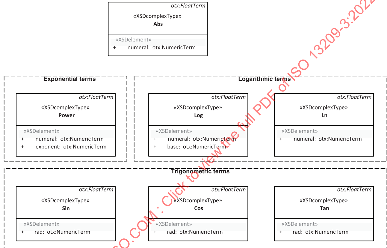
Figure 83 — Data model view: Math terms
