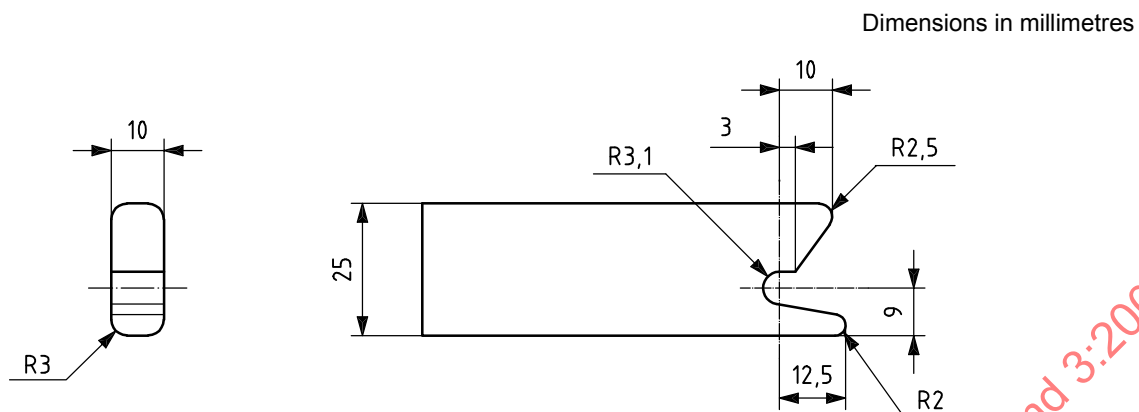
Figure 8.2 — Minimum dimensions of the connector
