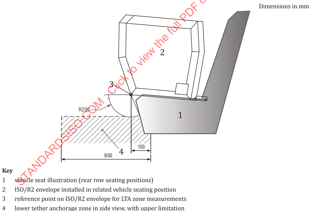
Figure 1 — Lower tether anchorage zone for rear seat row(s), side view
