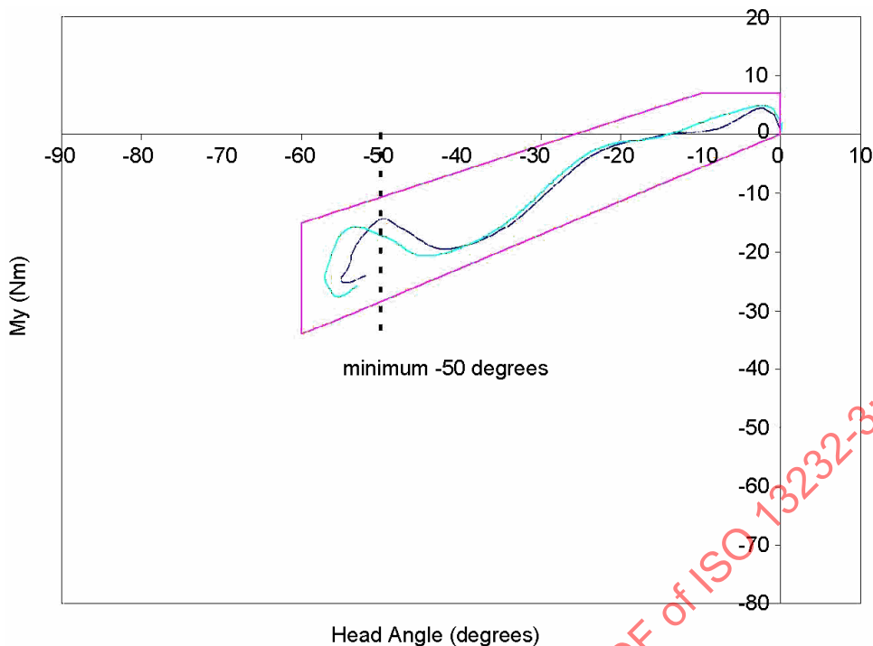
Figure 1 — Extension moment vs. head angle
