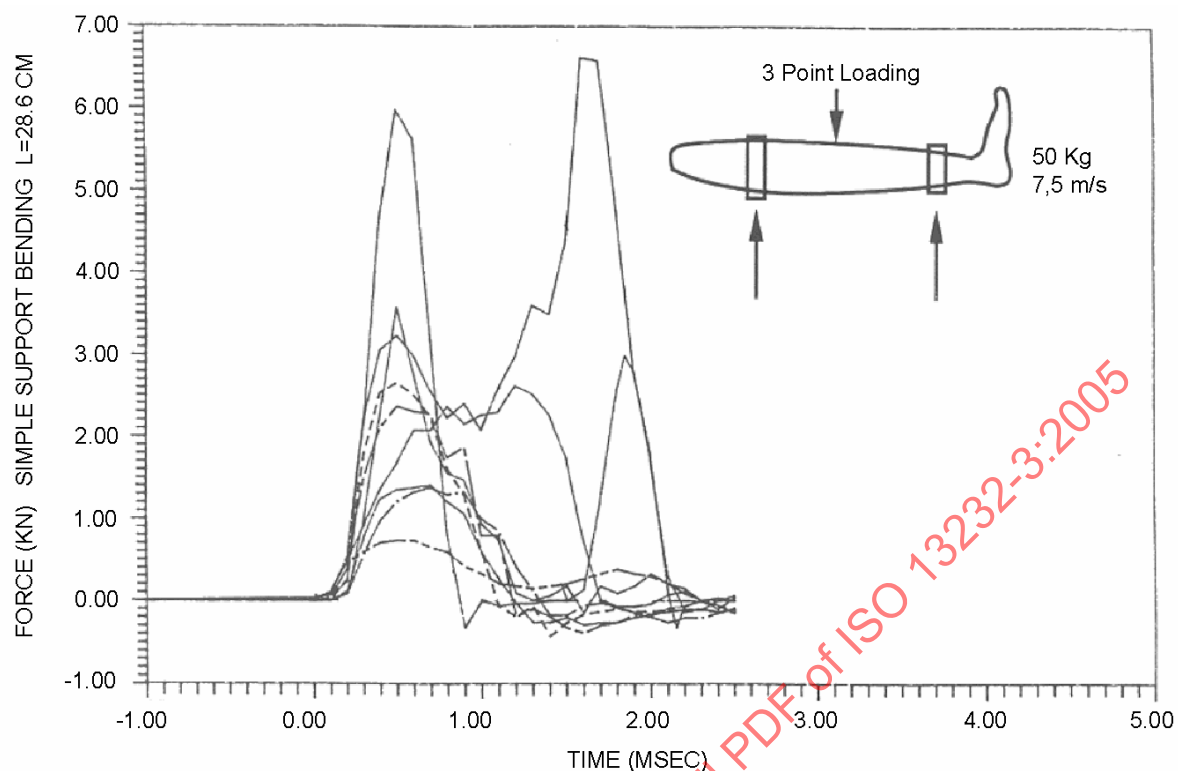
Figure B.19 — Impactor time histories for nine cadaver tibia specimens from Fuller and Snyder, 1989
