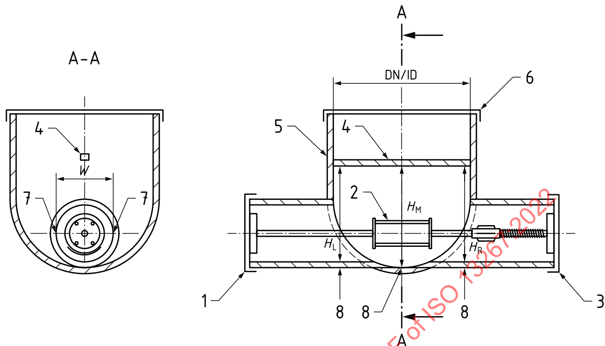
b) Spherical constructions with internal measuring points
