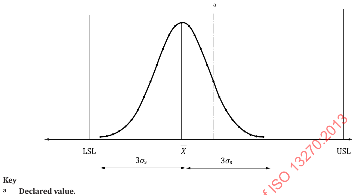
Figure 1 — Calculation of the Cpk-value
