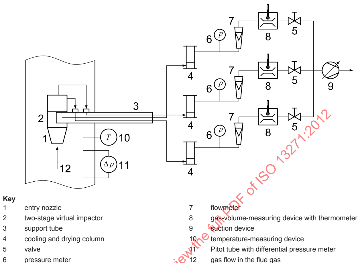
Figure 5 — Example of the design of the sampling system
