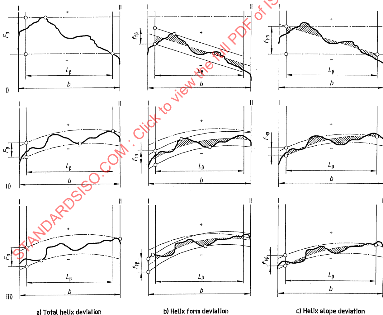
Figure 3 — Helix deviations
