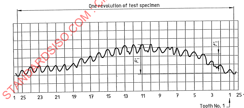
Figure 4 — Tangential composite deviations
