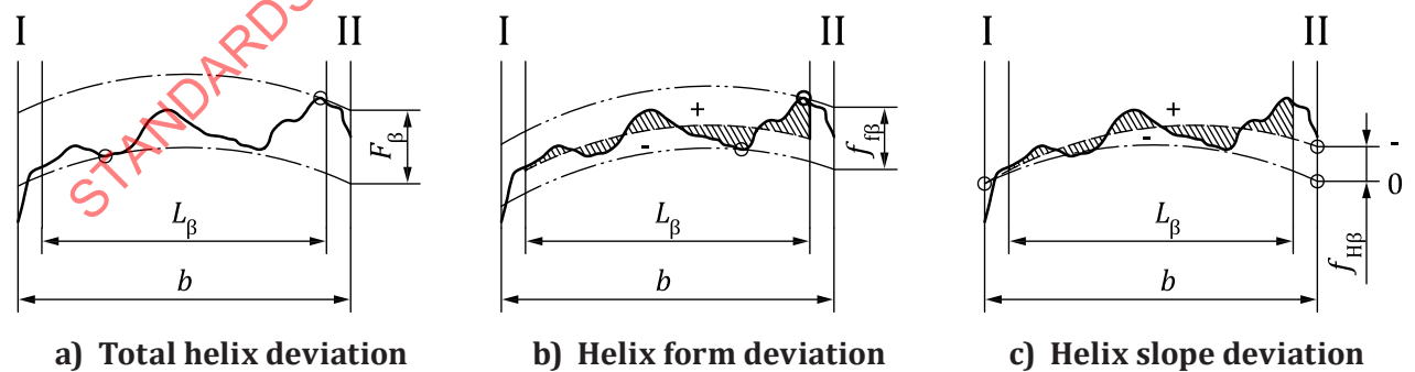
Figure 10 — Helix deviations with helix angle modification
