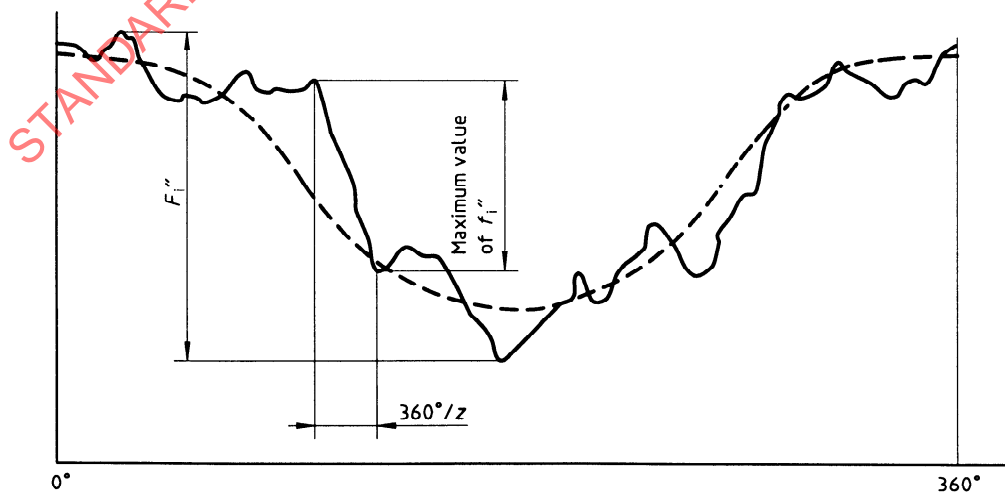
Figure 1 - Radial composite deviation diagram
