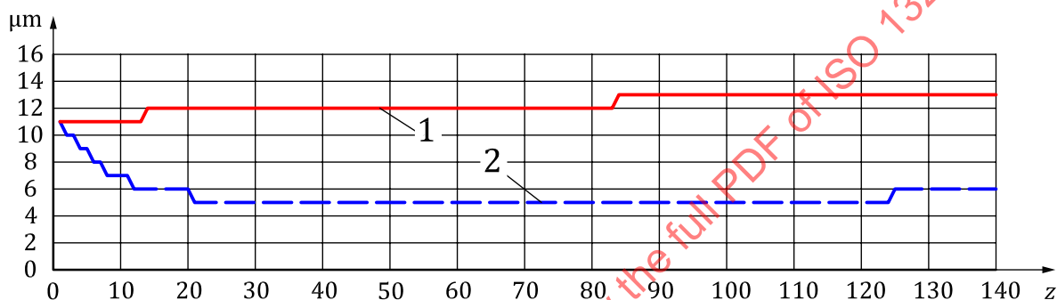
a) Double flank radial composite tolerance class 34
