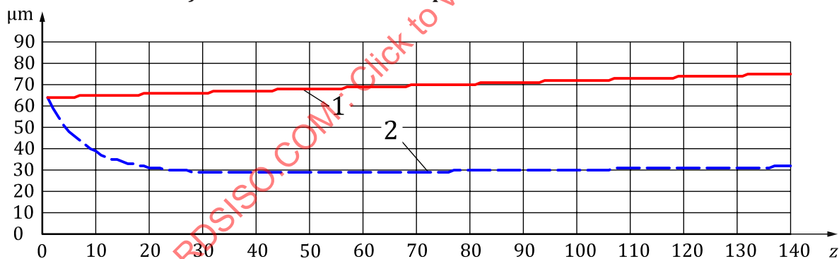
a) Double flank radial composite tolerance class 34
