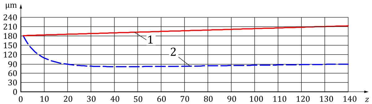
c) Double flank radial composite tolerance class 50
