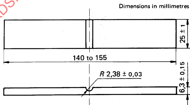
FIGURE 2 — Test piece
