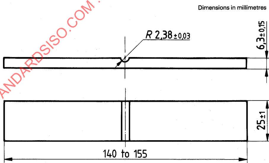
Figure 2 — Test piece
