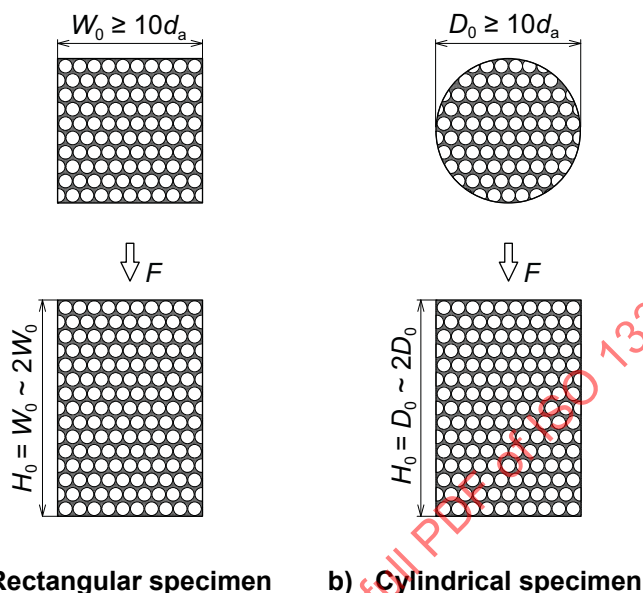
Figure 3 — Schematic illustration of test specimen
