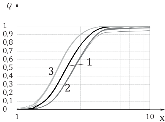
a) Extinction efficiency vs. particle size
