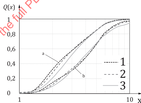
b) Exemplary result of multi-wavelength photo-sedimentation, conventional approach
