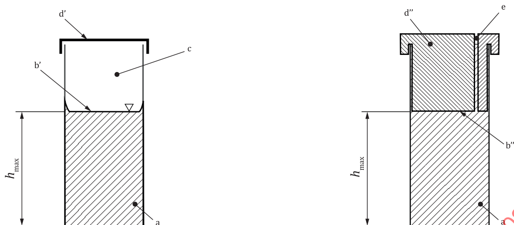
a) Cap-like lid design, which allows for an air buffer above the liquid sample
