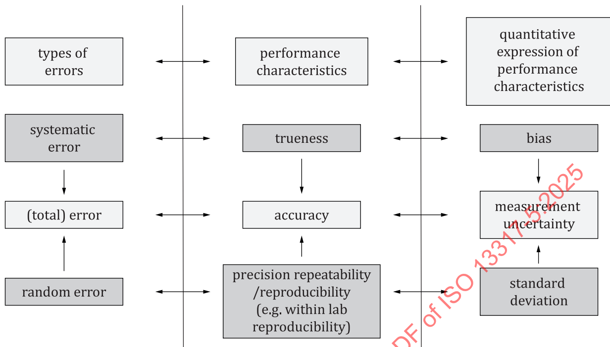
Figure 10 — Interrelations between error types, performance characteristics used to estimate them and expressions of quantitative estimates
