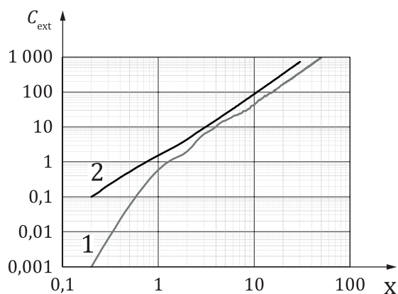
a) Extinction cross-section vs. particle size
