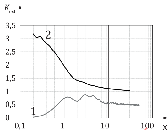
b) Extinction efficiency vs. particle size
