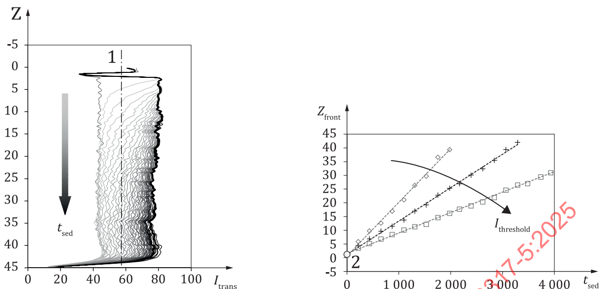
a) Evolution of profiles of the transmitted signals ( I_{\text{trans}} ) with indication of a signal threshold ( I_{\text{threshold}} ) used for front tracking
