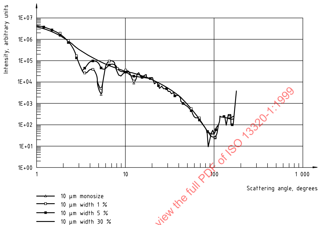
Figure A.6 — Influence of distribution width on angular light intensity scattering patterns of normal size distributions around 10 µm (particle RI = 1,62; medium water RI = 1,33)
