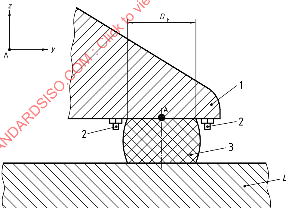
Figure 5 — Location of two accelerometers for measurement of \bar{L}_{vz}
