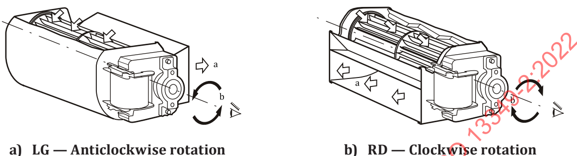
Figure 2 — Direction of rotation of axial-flow and mixed-flow fans
