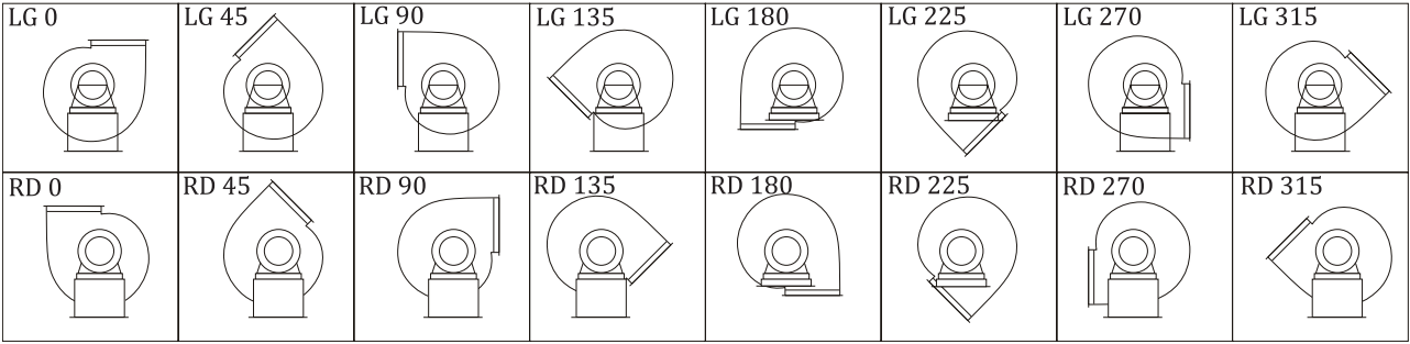
Figure 5 — Recommended positions for the outlet of a centrifugal fan
