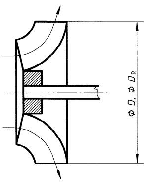
Figure 3 — Impeller of a mixed-flow fan
