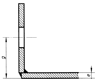
Fabricated flange design
