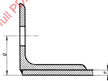
Lap-weld design
