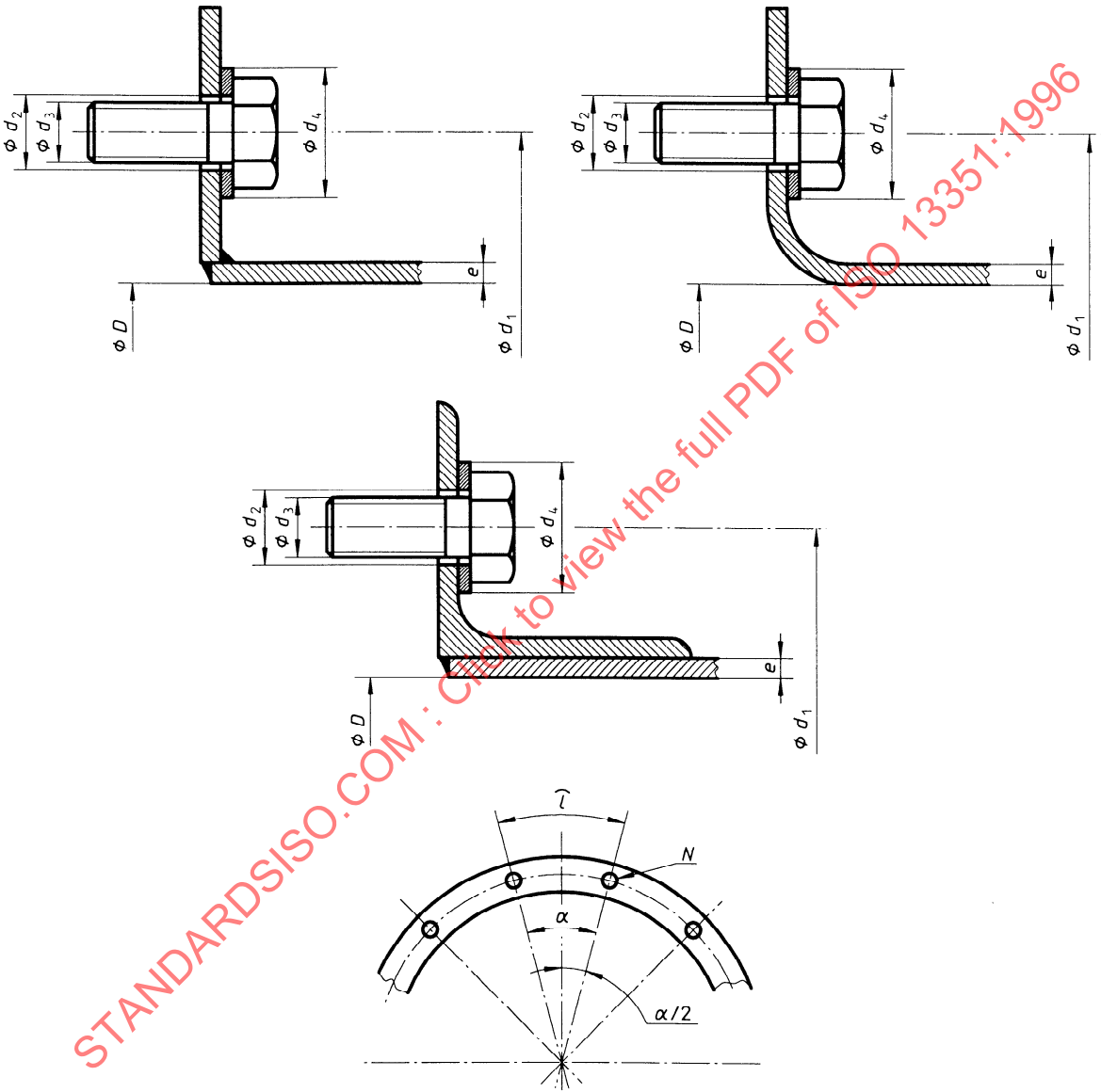
Figure 4 — Circular flanges
