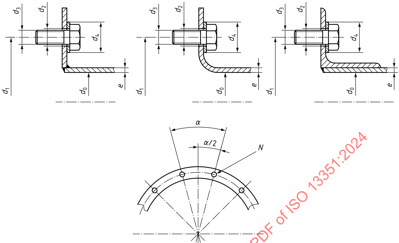
Figure 4 — Dimensions — Circular flanges
