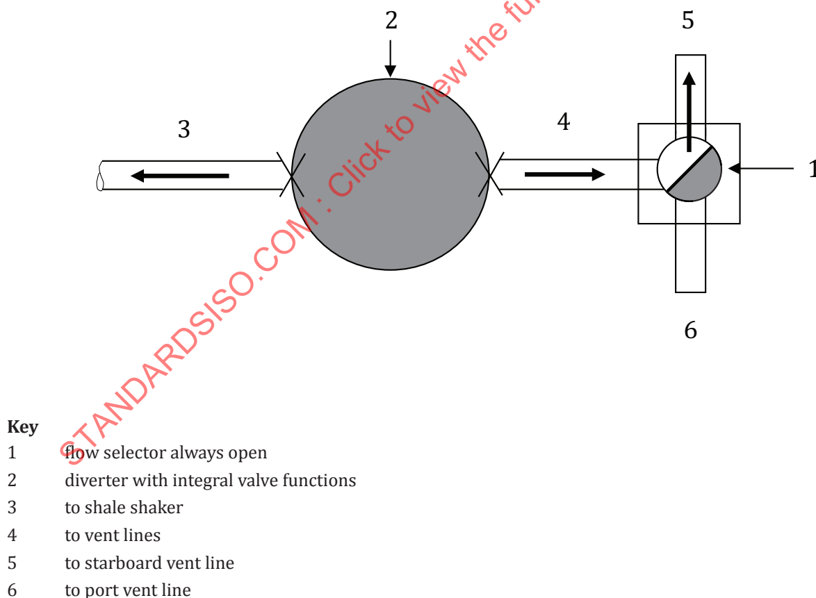
Figure 9 — Principle of flow selector system
