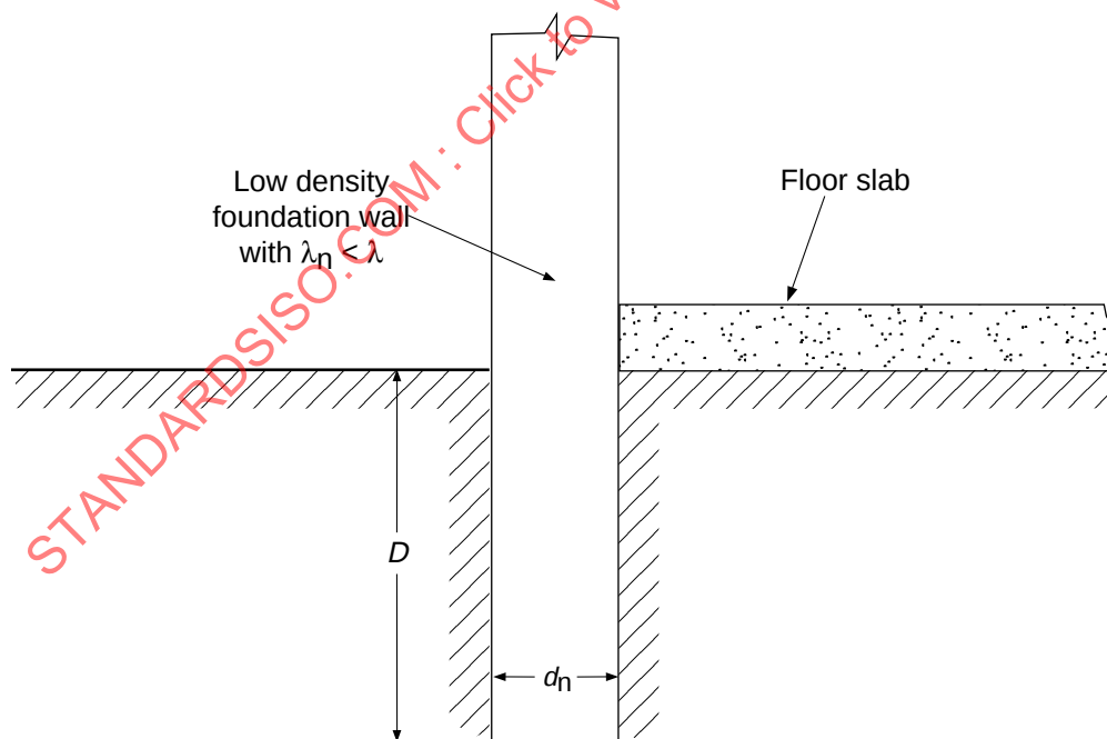
Figure 4 - Vertical edge insulation (low density foundation)
