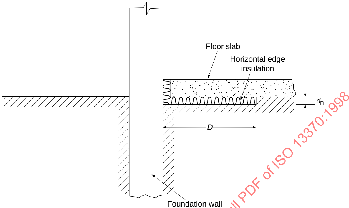
Figure 2 - Schematic diagram of horizontal edge insulation
