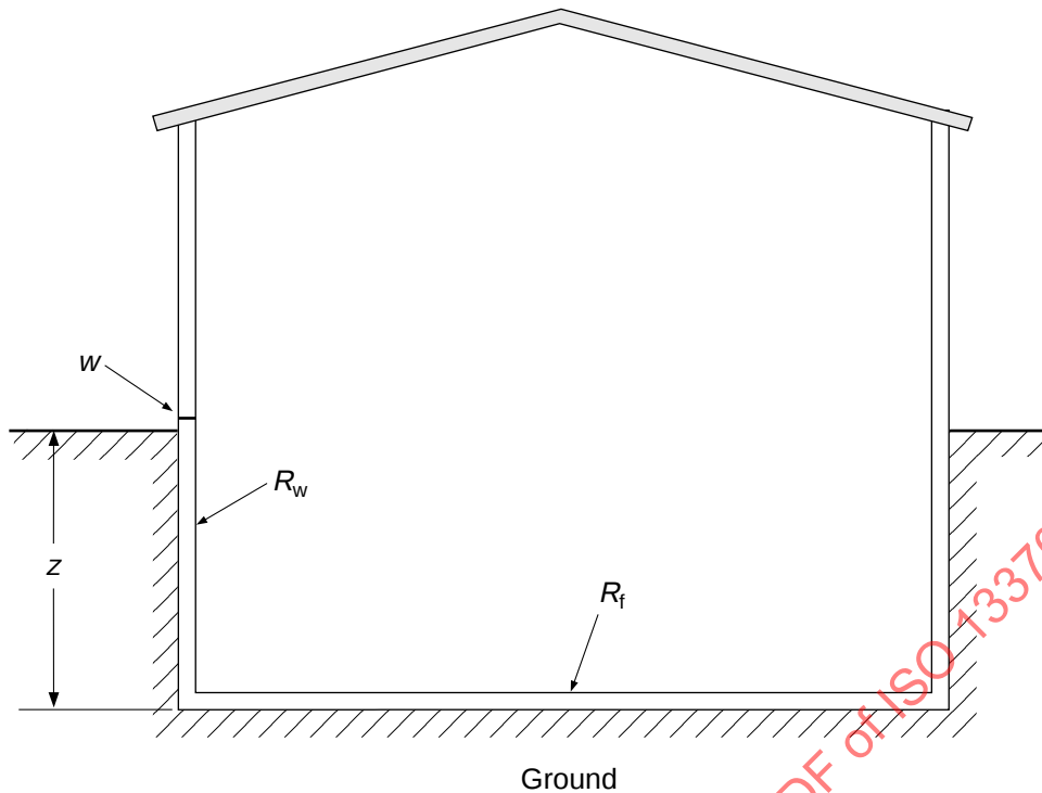
Figure 6 - Schematic diagram of building with heated basement
