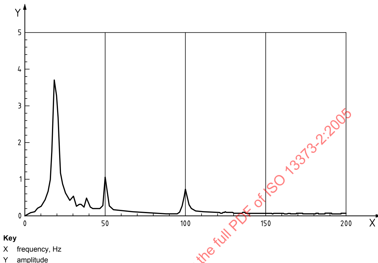
Figure 16 — Magnitude frequency spectrum
