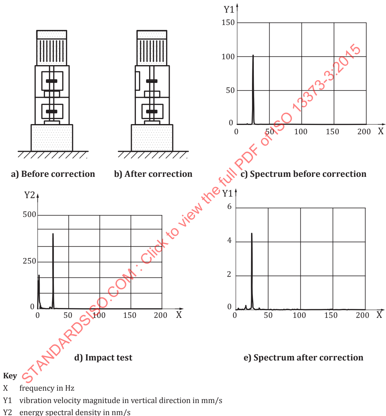
Figure B.4 — Resonance testing of a vertical pump
