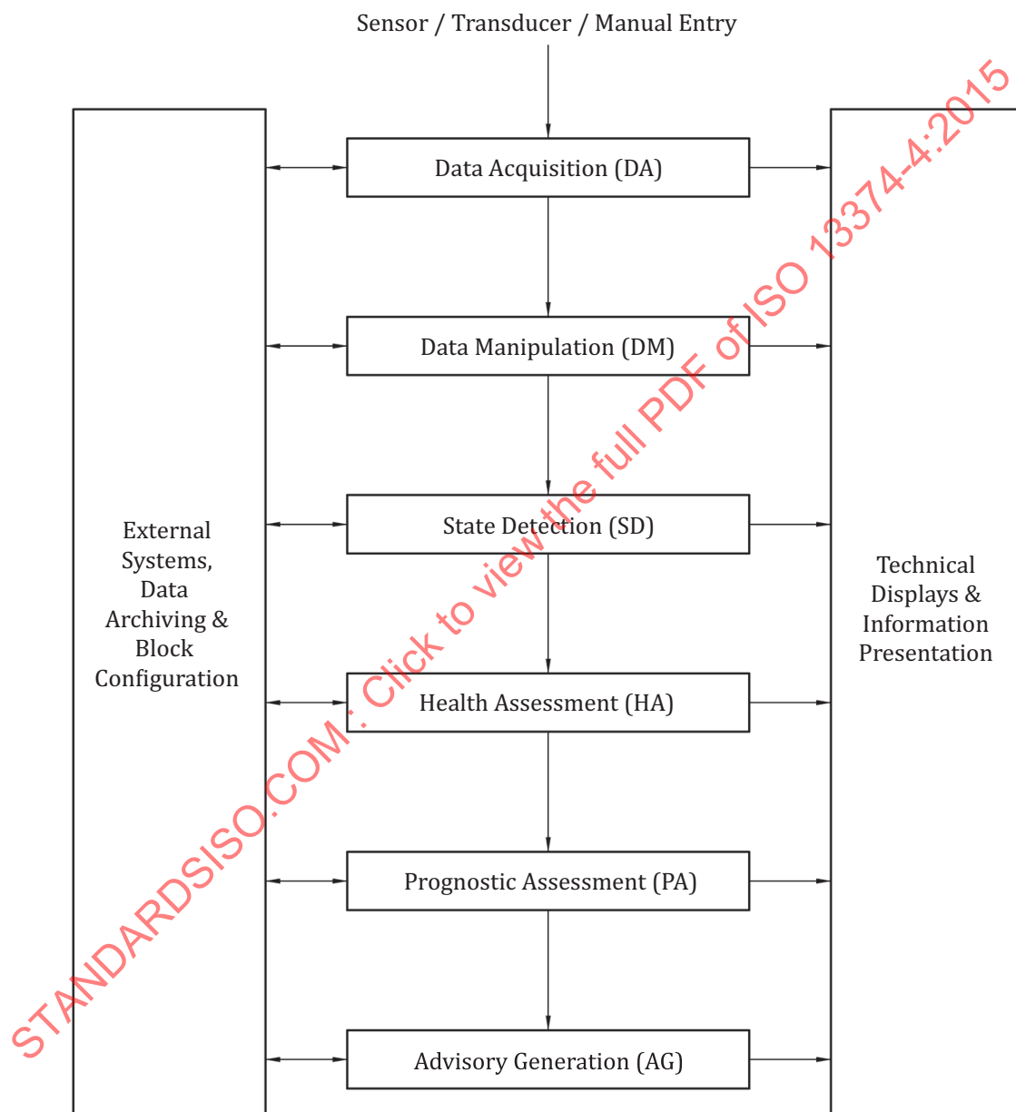
Figure 2 — Data processing block diagram (from ISO 13374-1:2003)
