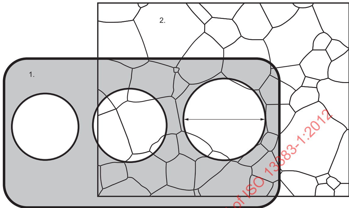
Figure 2 — Use of a stencil, 1, overlaid on a micrograph, 2, and visually matched to the selected grain being measured.
