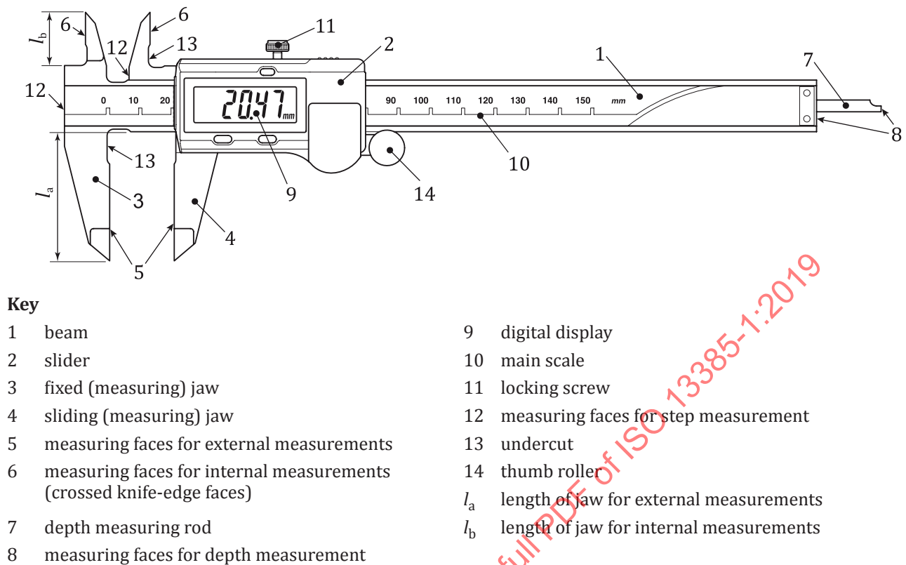
Figure 1 — Example design of callipers with digital display for external, internal, depth and step measurement
